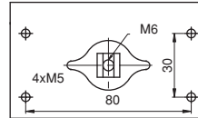
DETAIL "X"
